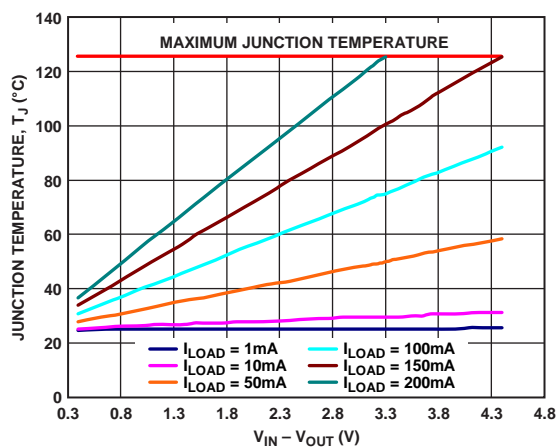
Figure 45. TSOT 50 mm 2 of PCB Copper, T A = 25°C
