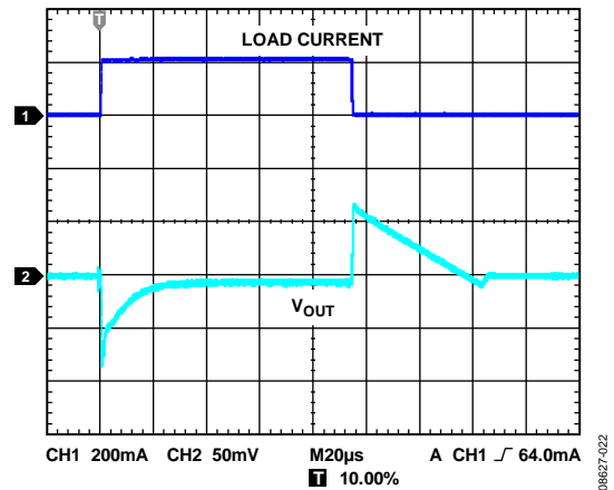
Figure 22. Load Transient Response, C_{IN}, C_{OUT} = 1\ \mu\text{F} , I_{LOAD} = 1\text{ mA to } 200\text{ mA}
