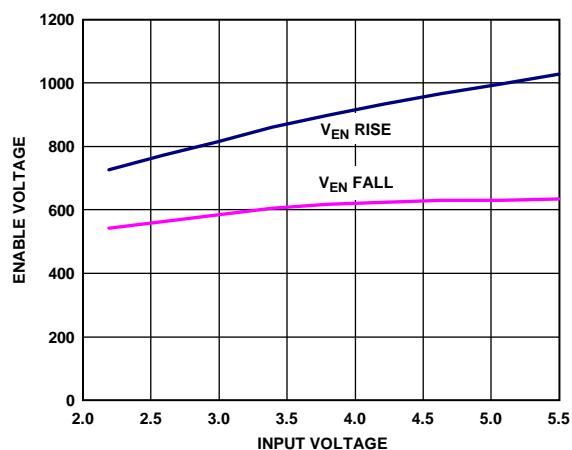
Figure 29. Typical EN Pin Thresholds vs. Input Voltage
